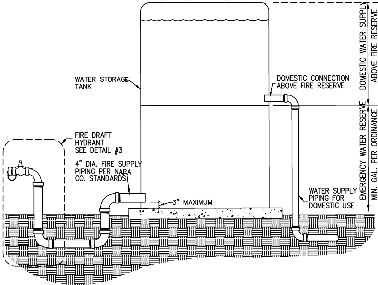
WATER STORAGE TANK
